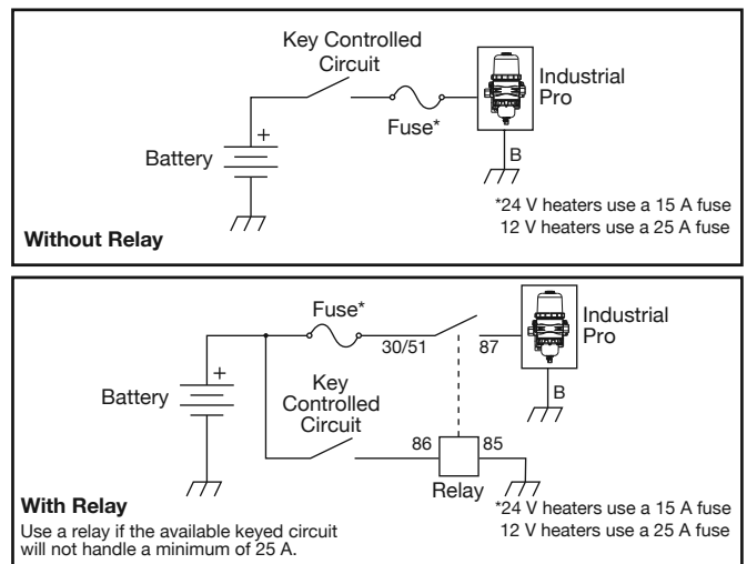
Figure 5 – Pre-heater Wiring Options
