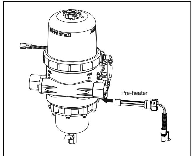
Figure 4 - Pre-heater Installation
