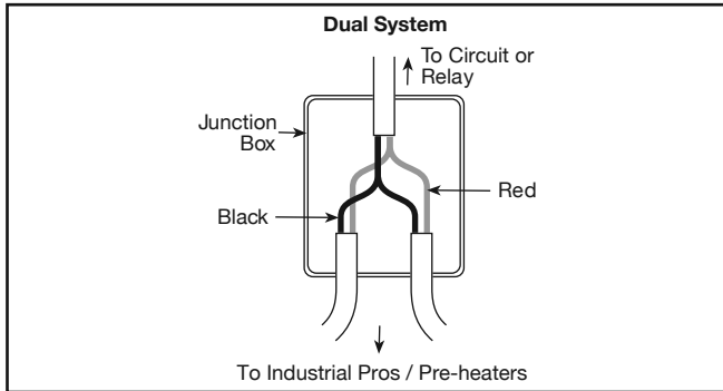
Figure 6 – Wiring Dual Filter Systems
